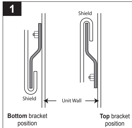
Bracket orientation to create top and bottom tracks
