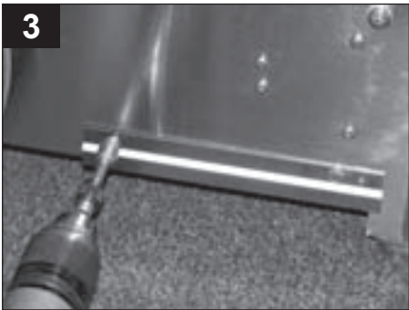
Remove and save bottom 2 screws. Place mounting bracket in correct position for lower track and install using existing screws. Repeat on opposite side.
