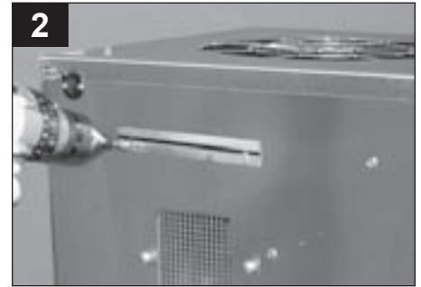
Remove and save rear 2 of 3 top screws. Place mounting bracket in correct position for upper track and using existing screws. Repeat on opposite side.
