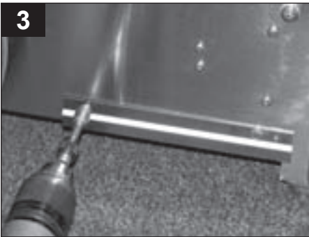
Remove and save bottom 2 screws. Place mounting bracket in correct position for lower track and install using existing screws. Repeat on opposite side.
